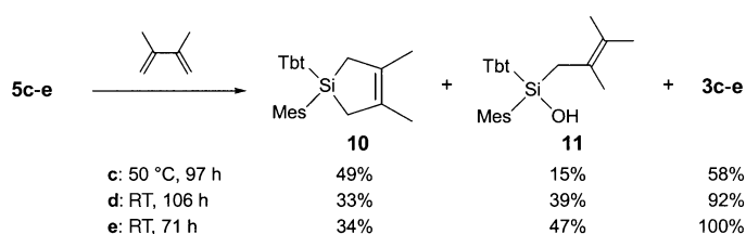
Scheme 10. Reaction of silylene–isocyanide complexes 5c–e with 2,3-dimethyl-1,4-butadiene.
