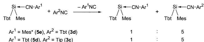
Scheme 8. Isocyanide-exchange reaction.
