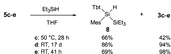
Scheme 7. Reaction of silylene–isocyanide complexes 5c–e with Et 3 SiH.
