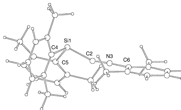
Figure 3. Optimized structure of 5f at the B3LYP/6–31G(d) level. Selective bond lengths [Å] and bond angles [ ^\circ ]: Si1–C2 1.867, Si1–C4 1.945, Si1–C5 1.918, C2–N3 1.184, N3–C6 1.373; Si1–C2–N3 159.35 , C2–Si1–C4 94.12 , C2–Si1–C5 110.43 , C4–Si1–C5 111.41 , C2–N3–C6 175.00 .
