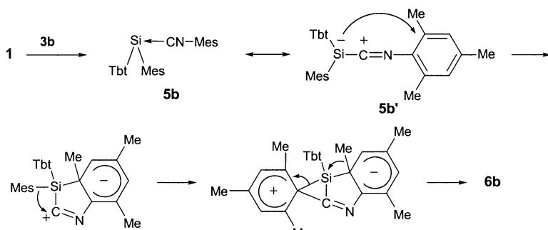
Scheme 5. Plausible mechanism for the formation of 6b .
