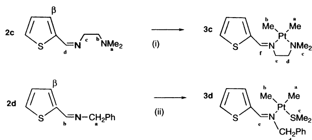
Scheme 2. (i) and (ii) Reactions with [Pt 2 Me 4 (μ-SMe 2 ) 2 ] ( 1 ) in acetone, (i) 16 h; (ii) 15 min.
