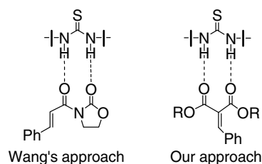
Fig. 1. Proposed hydrogen-bonding between the catalyst and the substrates.
