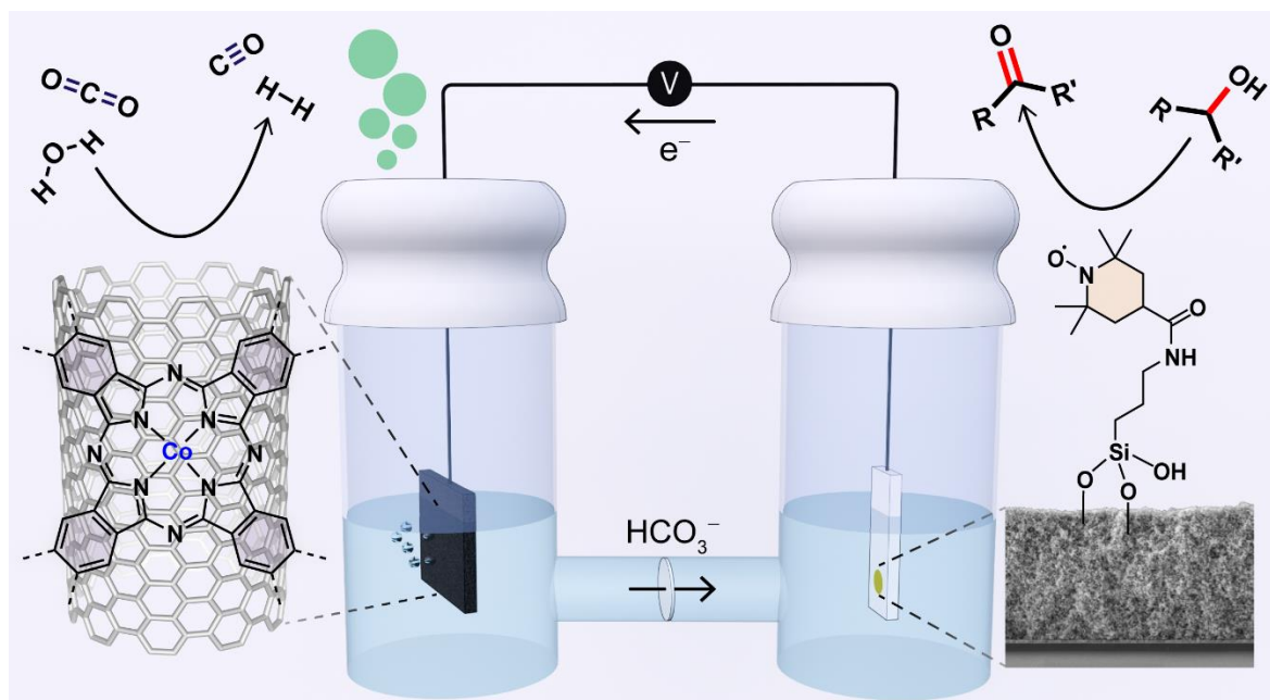
Figure 1: Coupled AlcOx-CO 2 R electrolyzer, featuring a meso ITO|STEMPO anode (right-hand compartment) and a CP|CNT-CoPPc cathode. An SEM cross-section image of the meso ITO electrode is shown on the right (film thickness ~4.5 μm).
