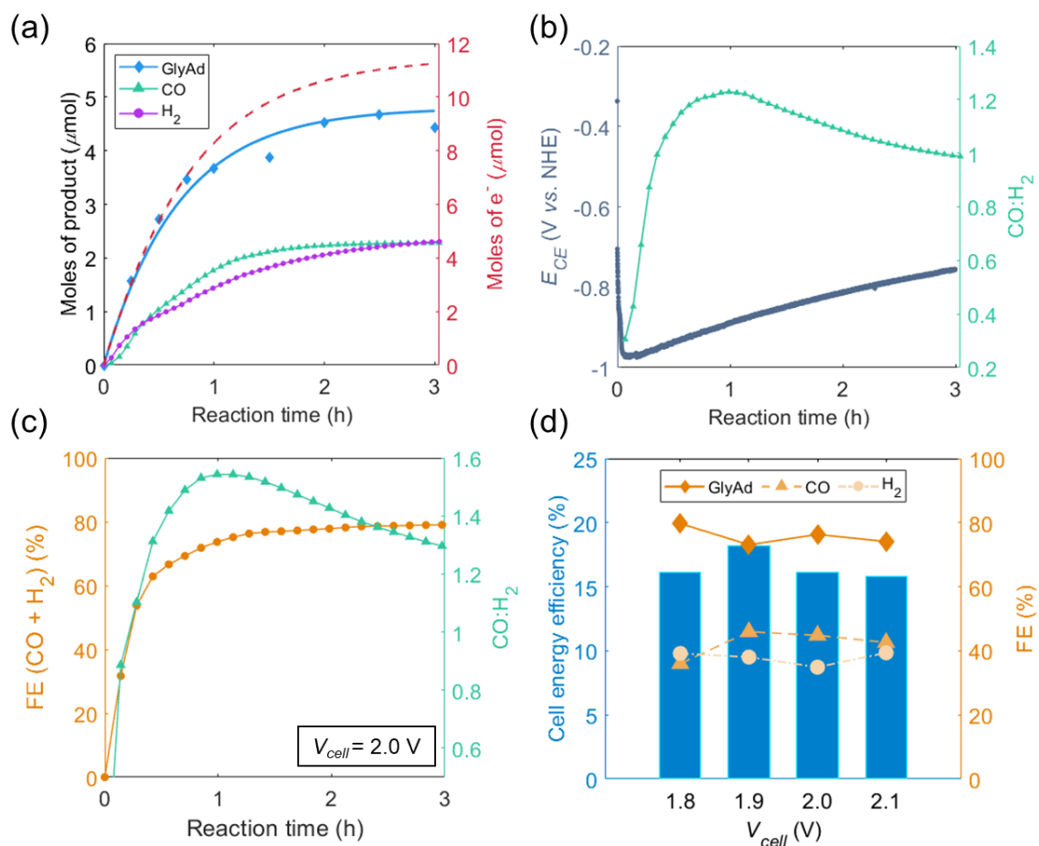
Figure 5: (a) Similar profile to Figure 4c, but with glycerol as the substrate ( E_{app} (anode) = 1 V vs. NHE). (b) Trend in the \text{CO}:\text{H}_2 ratio and CP|CNT-CoPPc CE potential ( E_{CE} ) over reaction time. (c) Combined FE for CO and \text{H}_2 , and \text{CO}:\text{H}_2 ratio for the two-electrode configuration incorporating glycerol as the substrate (applied cell potential = 2.0 V). (d) Cell energy efficiency and FE plotted as a function of V_{cell} in the same two-electrode setup. Conditions: for both the three-electrode (plots (a) and (b)), and two-electrode (plots (c) and (d)) configurations, a two-compartment cell (fitted with anion-exchange membrane) was used; anode compartment: \text{N}_2 saturated pH 8.3 aq. \text{HCO}_3^-/\text{CO}_3^{2-} (0.5 M); cathode compartment: \text{CO}_2 saturated pH 7.3 aq. \text{HCO}_3^-/\text{CO}_3^{2-} (0.5 M); glycerol substrate (50 mM) present in anodic compartment, t_{CPE} = 3 h. Glycerol oxidation and gaseous products quantified via HPLC and continuous flow GC analysis, respectively.
