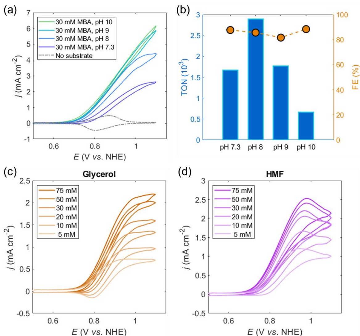
Figure 3: (a) pH dependent CVs measured for the meso |TO|STEMPO system, in the presence of 30 mM MBA. (b) TON and FE metrics compiled from the CPE experiment under a range of pH values. Conditions. pH 7.3: CO 2 saturated aq. HCO 3 - /CO 3 2- (0.5 M); pH 8 – 10: aq. HCO 3 - /CO 3 2- (0.5 M) titrated under ambient conditions to the correct pH; for CVs: \nu = 20 mV s -1 ; for CPE: E_{app} = 1 V vs. NHE, t_{CPE} = 3 h, MBA (30 mM). Product quantification (via HPLC) at the 3 h time-point was used for TON and FE calculation (Supporting Information, equations (S4) and (S5)). Electrochemically determined concentration profiles for (c) glycerol, and (d) HMF, using optimized pH (pH 8), and \nu = 20 mV s -1 .
