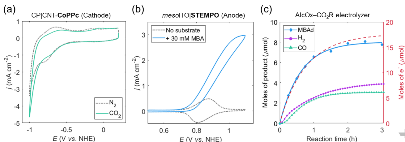
Figure 4: CVs for the (a) CP|CNT-CoPPc cathode, and (b) mesoITO|STEMPO anode, recorded separately in a three-electrode setup, with Pt mesh as the CE and Ag/AgCl as RE. Conditions: CO 2 saturated pH 7.3 aq. HCO 3 - /CO 3 2- (0.5 M), \nu = 20 \text{ mV s}^{-1} (pH 8 for cathode N 2 trace). (c) Coupled electrolyzer, showing moles of product (liquid and gaseous) and e - (as recorded on the potentiostat) over reaction time. Conditions: two-compartment cell fitted with anion-exchange membrane; three-electrode configuration with mesoITO|STEMPO as WE, CP|CNT-CoPPc as CE and Ag/AgCl as RE; CO 2 saturated pH 7.3 aq. HCO 3 - /CO 3 2- (0.5 M) in both compartments; MBA substrate (30 mM) present in anodic compartment, E_{app} (anode) = 1 V vs. NHE, t_{CPE} = 3 \text{ h} ; MBAd quantified by HPLC, CO/H 2 via continuous flow GC.
