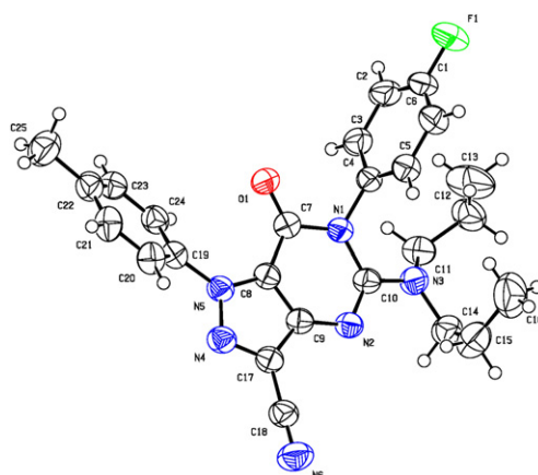
Figure 2. Crystal structure of 8h .
