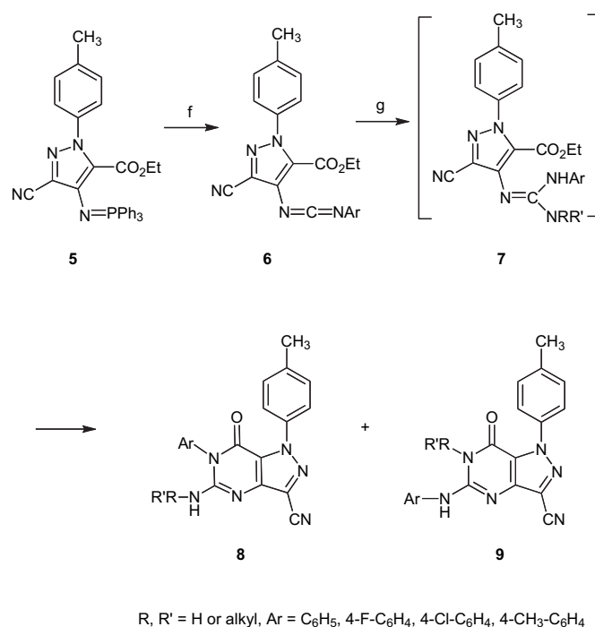
Scheme 2. Synthesis of 6-aryl-3-cyano-5-alkylamino-1- p -tolyl-1 H -pyrazolo[4, 3- d ]pyrimidin-7(6 H )-ones. Reagents and conditions: f. ArNCO, CH 2 Cl 2 , 0–5 °C, 12 h; g. RR'NH, CH 2 Cl 2 , rt, 6–12 h. When primary amine is used, 8 is the major product (73–96%), whereas when secondary amine is used, 8 is the sole product (70–97%).
