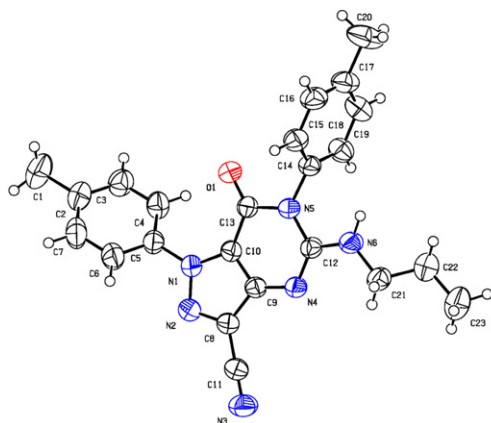
Figure 1. Crystal structure of 8u .
