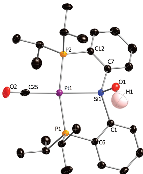
Figure 2. Crystal structure of complex 10 . The (\text{C}_6\text{F}_5)_4\text{B} -anion and all the hydrogen atoms except hydroxyl were omitted for clarity. The thermal ellipsoids are at 50% probability level.
