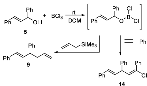
SCHEME 8. Evidence Supporting the Cleavage of the C–O Bond via BCl 3
