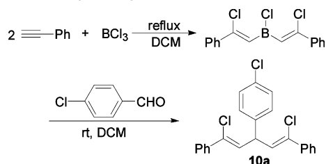
SCHEME 5. Reaction of (Z,Z)-Dialkenylboron Chloride with 4-Chlorobenzaldehyde
