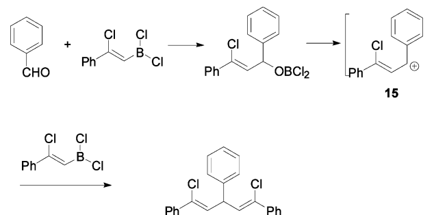
SCHEME 9. Reaction of Z -Chlorovinylboron Dichloride with Aldehyde
