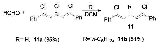
SCHEME 6. Dialkenylation of Aliphatic Aldehydes Using Preformed Divinylboron Halides
