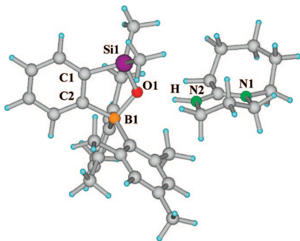
Figure 2. Optimized structure of 6 at the HF/6-31+G(d) level. Selected bond lengths (Å) and angles (deg): C1–C2, 1.4042; Si1–C1, 1.8357; Si1–O1, 1.6449; B1–O1, 1.5745; B1–C2, 1.6721; O1···N2, 2.8605; O1···H, 1.8451; C2–C1–Si1, 107.85; C1–Si1–O1, 97.78; Si1–O1–B1, 114.98; O1–B1–C2, 102.37; C1–C2–B, 115.88.
