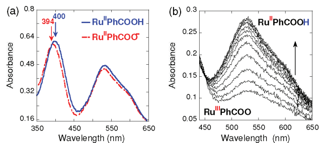
Figure 1. (a) UV–vis spectra [ \lambda /nm ( \epsilon /M -1 cm -1 )] for Ru II PhCOOH [400 (20 000), 533 (15 000)] and Ru II PhCOO - [394 (20 000), 531 (15 000)], each 0.030 mM in MeCN; \epsilon 's all \pm 1000 . 9 (b) Spectra for Ru II PhCOO (0.026 mM) + TEMPOH (0.20 mM) in MeCN over 0.5 s, showing the growth of Ru II PhCOOH .
