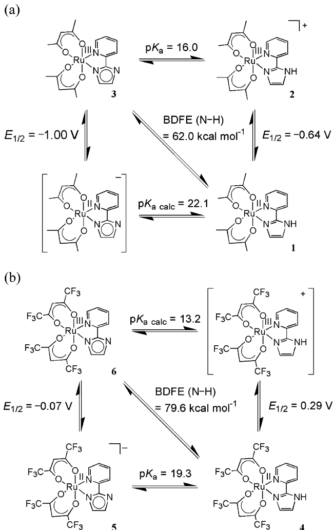
Scheme 2. Square Schemes for (a) the \text{Ru} -acac-py-imH ( 1–3 ) and (b) the \text{Ru} -hfac-py-imH ( 4–6 ) Systems (in MeCN at 298 K, E_{1/2} Values vs \text{Cp}_2\text{Fe}^{+/0} ).
