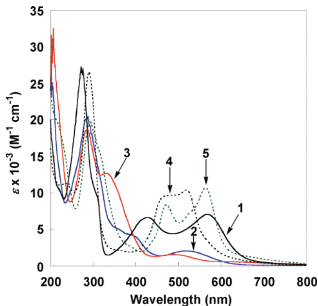
Figure 4. UV-vis spectra of \text{Ru}^{\text{II}}(\text{acac})_2(\text{py-imH}) ( 1 ), [\text{Ru}^{\text{III}}(\text{acac})_2(\text{py-imH})]\text{OTf} ( 2 ), \text{Ru}^{\text{III}}(\text{acac})_2(\text{py-im}) ( 3 ), \text{Ru}^{\text{II}}(\text{hfac})_2(\text{py-imH}) ( 4 ), and [\text{DBU-H}][\text{Ru}^{\text{II}}(\text{hfac})_2(\text{py-im})] ( 5 ) in MeCN.
