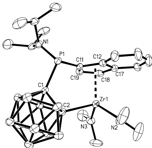
Figure 1. Molecular structure of [\eta^5:\sigma\text{-}^i\text{Pr}_2\text{NP}(\text{C}_9\text{H}_6)\text{-(C}_2\text{B}_{10}\text{H}_{10})]\text{Zr}(\text{NMe}_2)_2 ( 2 ).
