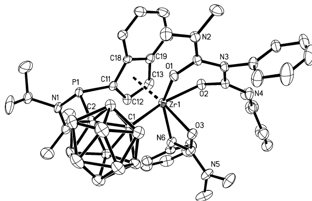
Figure 3. Molecular structure of [\eta^5:\sigma\text{-}^i\text{Pr}_2\text{NP}(\text{C}_9\text{H}_6)\text{-(C}_2\text{B}_{10}\text{H}_{10})]\text{Zr}[\eta^2\text{-OC}(\text{NMe}_2)\text{NPh}]\text{-}[\eta^2\text{-OC}(\text{NMe}_2)\text{N(Ph)C}=\text{(NPh)O}] ( 5 ) (the solvated \text{CH}_3\text{CN} molecule is not shown). Selected bond distances (Å) and angles (deg): Zr1–C1 = 2.401(5), Zr1–C11 = 2.666(5), Zr1–C12 = 2.456(5), Zr1–C13 = 2.480(5), Zr1–C18 = 2.675(5), Zr1–C19 = 2.653(5), av Zr1–C(ring) = 2.586(5), Zr1–O1 = 2.124(3), Zr1–O2 = 2.104(3), Zr1–O3 = 2.161(3), Zr1–N6 = 2.186(4), Cent–Zr1–C1 = 92.6, C2–P–C11 = 98.2(2).
