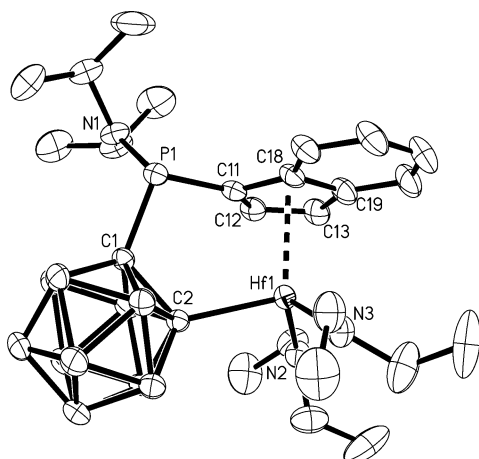
Figure 2. Molecular structure of [\eta^5:\sigma\text{-}^i\text{Pr}_2\text{NP}(\text{C}_9\text{H}_6)\text{-(C}_2\text{B}_{10}\text{H}_{10})]\text{Hf}(\text{NEt}_2)_2 ( 4 ).
