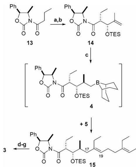
Scheme 4. Reagents and conditions: (a) \text{Bu}_2\text{BOTf} , (i\text{-Pr})_2\text{NEt} , methacrolein, \text{CH}_2\text{Cl}_2 , -78^\circ\text{C} , 95%; (b) \text{TESCl} , imidazole, DMF, rt, 98%; (c) 14 (3.0 equiv), 9-BBN dimer (3.0 equiv), THF, 0^\circ\text{C} , then \text{Cs}_2\text{CO}_3 (3.0 equiv), 10 mol % \text{Pd}(\text{dppf})\text{Cl}_2 , 5 (1.0 equiv), THF/1,4-dioxane/ \text{H}_2\text{O} = 10:8:1, rt, 82%; (d) \text{EtSH} , n\text{-BuLi} , THF, -78^\circ\text{C} , 91%; (e) \text{DIBALH} , \text{CH}_2\text{Cl}_2 , -78^\circ\text{C} , 92%; (f) \text{EtMgBr} , THF, -78^\circ\text{C} , 94%; (g) Dess–Martin periodinane, \text{CH}_2\text{Cl}_2 , 98%.
