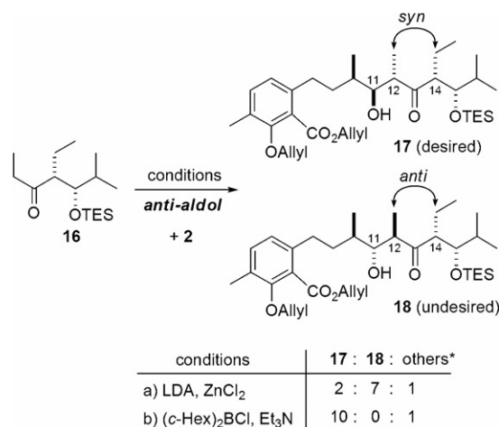
Scheme 5. Reagents and conditions: (a) (i) LDA (1.5 equiv), \text{Et}_2\text{O} , 0^\circ\text{C} , 30 min, (ii) \text{ZnCl}_2 (1.5 equiv), 0^\circ\text{C} , 30 min, (iii) 2 (1.0 equiv), \text{Et}_2\text{O} , 0^\circ\text{C} , 10 min, 17 (12%), 18 (42%), 16 (15% recovery); (b) (c\text{-Hex})_2\text{BCl} (1.2 equiv), \text{Et}_3\text{N} (1.2 equiv), then 2 (1 equiv), THF, -78^\circ\text{C} , 17 (27%), 16 (42% recovery). *Mixture of other aldol adducts.
