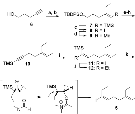
Scheme 3. Reagents and conditions: (a) TBDPSCl, imidazole, DMF, 98%; (b) Et 2 Zn, TMSI, 5 mol % Pd(PPh 3 ) 4 , 1,4-dioxane, 45%; (c) NIS (1.2 equiv), CH 3 CN, 95%; (d) ZnCl 2 , MeMgBr, Pd(PPh 3 ) 4 , THF, 96%; (e) Bu 4 NF, THF; (f) (COCl) 2 , DMSO, Et 3 N, CH 2 Cl 2 , –78 to –45 °C; (g) CBr 4 , PPh 3 , pyridine, CH 2 Cl 2 , 53% (three steps); (h) n -BuLi, TMSCl, THF, –78 °C, 95%; (i) Cp 2 ZrCl 2 (1.5 equiv), DIBALH (1.5 equiv), then NIS (1.2 equiv), THF, 10 °C, 69%; (j) EtMgBr, ZnCl 2 , Pd(PPh 3 ) 4 , THF, 99%; (k) NIS (1.2 equiv), DMF, 53%.
