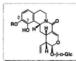
Neoalangiside ( 1 ): R=Me Demethylneoalangiside ( 2 ): R=H
