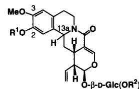
Alangiside ( 3 ): H13a ( \beta ), R 1 =R 2 =H 4 : H13a ( \beta ), R 1 =Me, R 2 =Ac 5 : H13a ( \alpha ), R 1 =Me, R 2 =Ac
