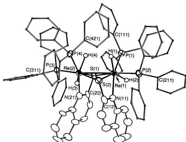
Figure 1. ORTEP 33 representation of the structure of the dirhenium cation [\text{Re}_2\text{H}_4(\mu\text{-mq})_2(\text{PPh}_3)_4]^{2+} present in complex 4a . The thermal ellipsoids are drawn at the 50% probability level except for those of the hydrido ligands and the phenyl group atoms of the \text{PPh}_3 ligands, which are circles of arbitrary radius.
