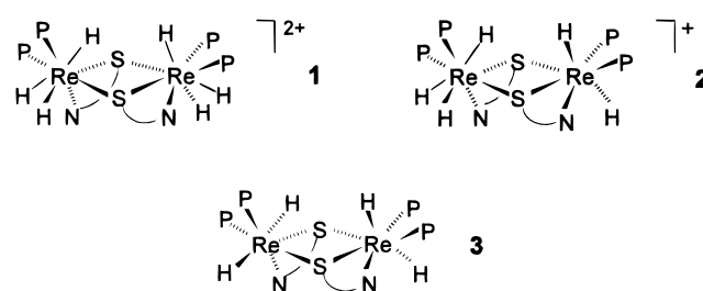
Chart 1. Representation of the Structural Relationships among 1 – 3
