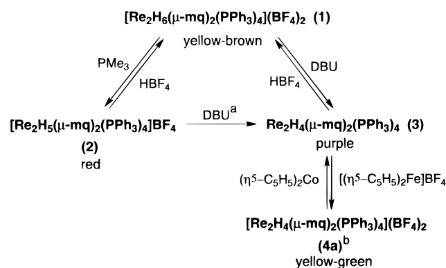
Scheme 1. Reaction Chemistry of [\text{Re}_2\text{H}_6(\mu\text{-mq})_2(\text{PPh}_3)_4](\text{BF}_4)_2 ( 1 )
