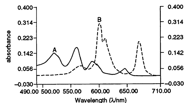
Fig. 2 Visible or Q band region of the electronic spectra for 4b (A) and 4a (B) in dichloromethane. The Soret bands for 4b and 4a appear at 416 and 438 nm, respectively, which are omitted.
