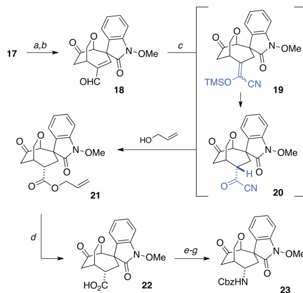
Scheme 3. Pivotal, Stereoselective Introduction of a Nitrogen Atom a
