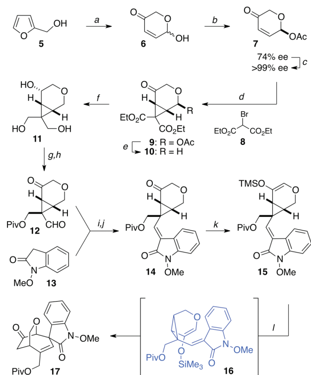
Scheme 2. Divinylcyclopropane–Cycloheptadiene Rearrangement a
