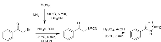
Scheme 5 One pot radiolabelling of 4-phenylthiazol-2- ^{11}\text{C} one (10) via acid mediated cyclisation of the intermediate 1-phenyl-2- ^{11}\text{C} thiocyanatoethanone (2), (*) denotes the ^{11}\text{C} labelling position.
