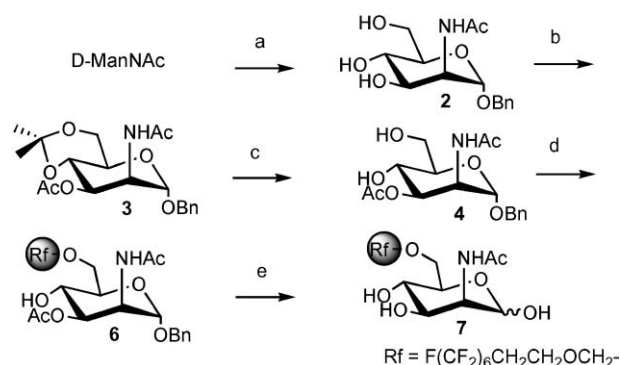
Scheme 2 Reagents and conditions: (a) (i) \text{Ac}_2\text{O} , pyridine, \text{CH}_2\text{Cl}_2 , rt, 24 h, (ii) \text{BnOH} , \text{BF}_3 \cdot \text{OEt}_2 , \text{CH}_3\text{NO}_2 , 80 °C, 7 h, (iii) \text{NaOMe} , \text{MeOH} , 0 °C, 3 h, 68% from D-ManNAc; (b) (i) 2,2-dimethoxypropane, PTSA, \text{DMF} , rt, 1 h, (ii) \text{Ac}_2\text{O} , pyridine, rt, 24 h, 84% from 2 ; (c) 80% \text{AcOH} , 80 °C, quant.; (d) \text{RfCl} 5 , \text{Pr}_2\text{NEt} , \text{DMF} , 45 °C, 54 h, 81%; (e) (i) \text{NaOMe} , \text{MeOH} , 0 °C, 2 h, (ii) 20% \text{Pd}(\text{OH})_2/\text{C} , \text{H}_2 , \text{MeOH} , rt, 24 h, 94% from 6 .
