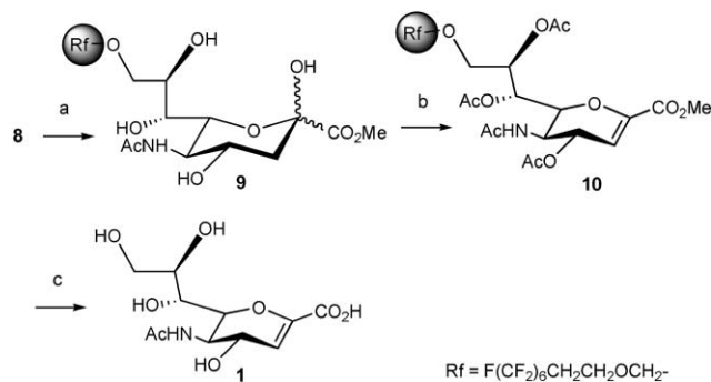
Scheme 3 Reagents and conditions: (a) \text{TMSCHN}_2 , \text{CH}_2\text{Cl}_2 , rt, 24 h, quant. from 8 ; (b) (i) \text{AcCl} , rt, 24 h; (ii) pyridine, rt, 1 h, 87% from 9 ; (c) (i) \text{NaOMe} , \text{MeOH} , 0 °C, 2 h; (ii) \text{TMSBr} , \text{CH}_2\text{Cl}_2 , 0 °C, 12 h, 67% from 10 .
