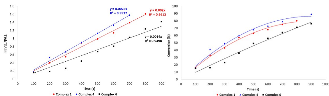
Figure 7. Left: Plot of \ln[VL]_0/[VL]_t vs. time using complex 1 , 4 and 6 ; right: relationship between conversion and time for the polymerization of VL.
