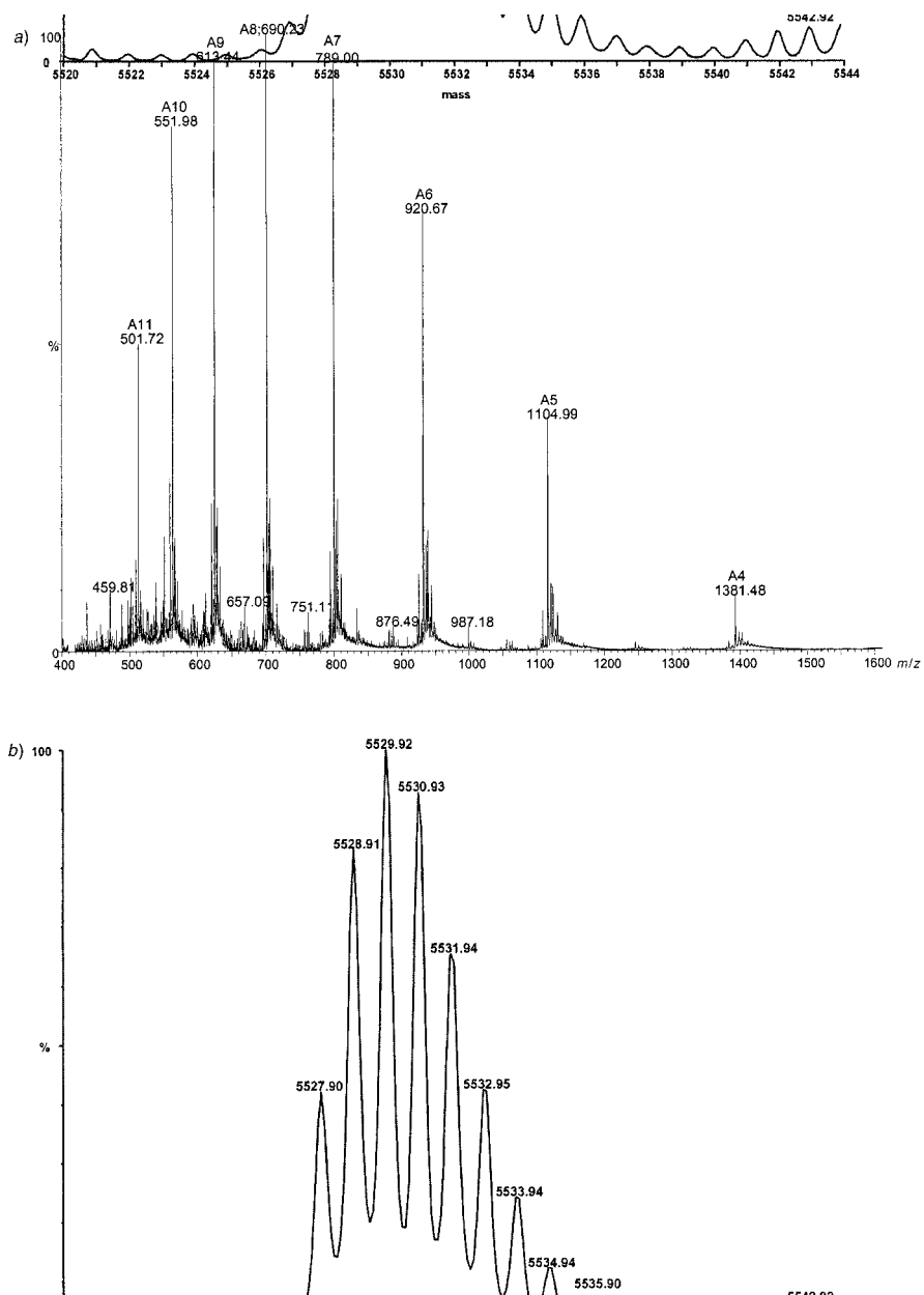
Fig. 2. a) ESI-Mass spectrum of the RNA 17-mer corresponding to the anticodon loop of tRNA Met in which the adenine base at position 11 is replaced by N-[(9-( \beta -D-ribofuranosyl)-9H-purin-6-yl]carbamoyl-L-threonine (t 6 A) and b) its Max Ent 1 processed spectrum, indicating the experimental monoisotopic mass. See Exper. Part for details.
