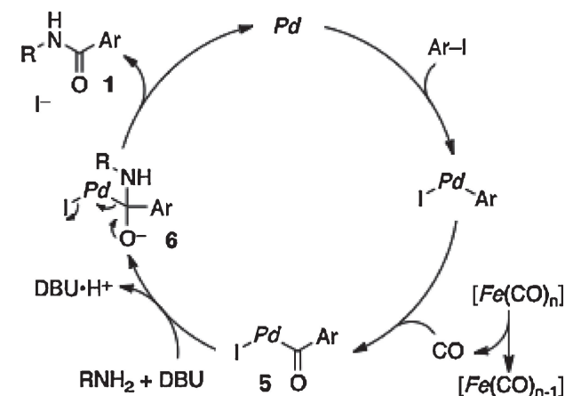
Scheme 1. Plausible reaction mechanism.
