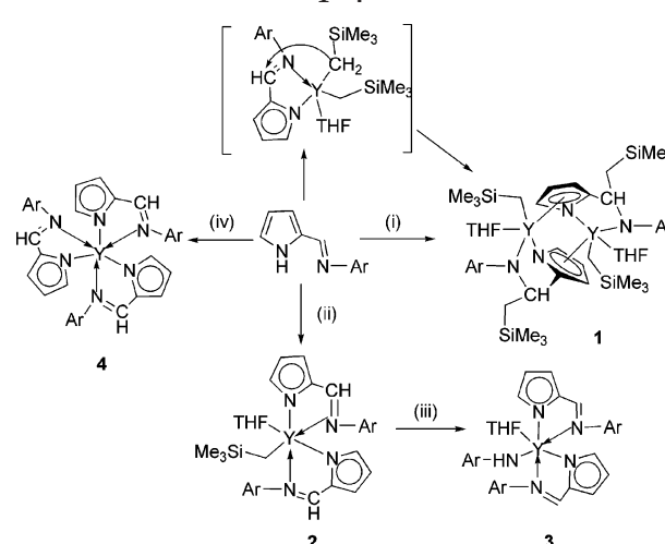
Scheme 1 . Synthetic Pathway for Preparation of Complexes 1–4 a
