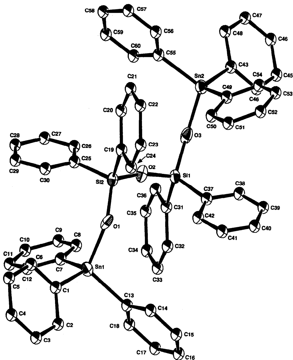
Fig. 1. The asymmetric unit of (\text{Ph}_3\text{SnO})\text{Ph}_2\text{SiOSiPh}_2(\text{OSnPh}_3) , showing the labelling scheme used in the text and tables. Thermal ellipsoids for the Sn, Si and O atoms are at the 30% probability level.
