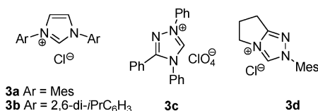
Figure 1. Structures of azolium salts 3 .
