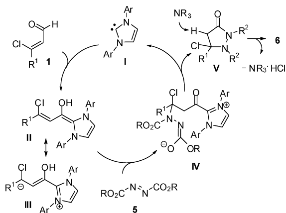
Scheme 3. Plausible Mechanism of the Reaction of 1 and 5 (NR 3 = DBU; Ar = 2,6-di- i PrC 6 H 3 )
