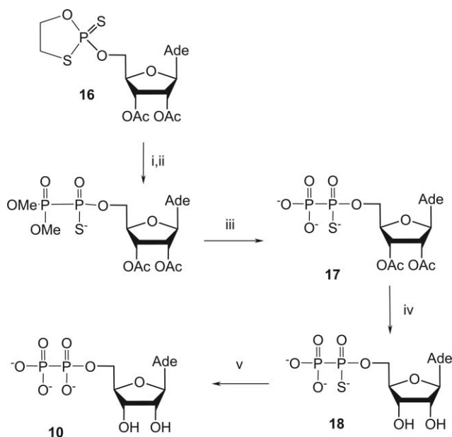
Scheme 6 Synthesis of adenosine 5'-O-(P 1 -thiohypophosphate) and hypophosphate derivatives. Reagents: (i) (MeO) 2 P(O)H; (ii) DBU; (iii) TMS-Br; (iv) NH 4 OH aq ; (v) PhIO 2 .
