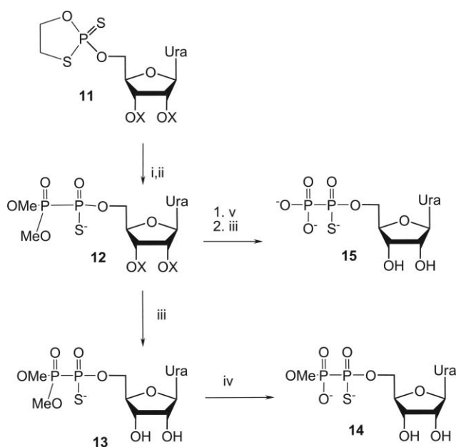
Scheme 5 Synthesis of uridine 5'-O-(P 1 -thiohypophosphate) derivatives. X = isopropoxyacetyl. Reagents: (i) (MeO) 2 P(O)H; (ii) DBU; (iii) NH 4 OH aq ; (iv) t -Bu-NH 2 ; (v) TMS-Br.
