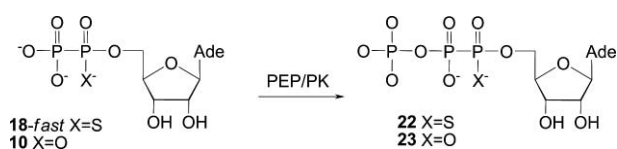
Scheme 8 Enzymatic conversion of adenosine 5'- O -( \text{P}^1 -thiohypophosphate) or 5'- O -hypophosphate into the corresponding \text{P}^1 , \text{P}^2 -hypotriphosphate analogues ( 22 or 23 ) of ATP \alpha S or ATP, respectively. PEP/PK, phosphoenolpyruvate/pyruvate kinase.
