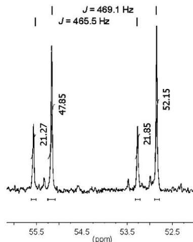
Fig. 1 A region of the 31 P NMR spectrum for the P 1 atoms in both P-diastereomers of 5'-O-DMT- N 1Bu , O DPC -deoxyguanosine-3'-O-(P 2 ,O,O-diethyl-P 1 -thiohypophosphate) ( 20 ). The vertical numbers represent integration data.
