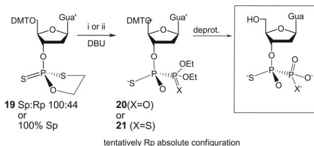
Scheme 7 Synthesis of stereodefined nucleoside 3'-O-(P 1 -thiohypophosphate) or 3'-O-(P 1 ,P 2 -dithiohypophosphate). Gua' = Gua 1Bu,DPC ; Reagents: X = O, (i) (EtO) 2 P(O)H; X = S, (ii) (EtO) 2 P(S)H. (The major S P isomer of 19 is shown.).
