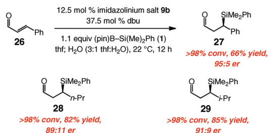
Scheme 4. NHC-Catalyzed Enantioselective Silyl Conjugate Addition (SCA) Reactions with \alpha,\beta -Unsaturated Aldehydes a
