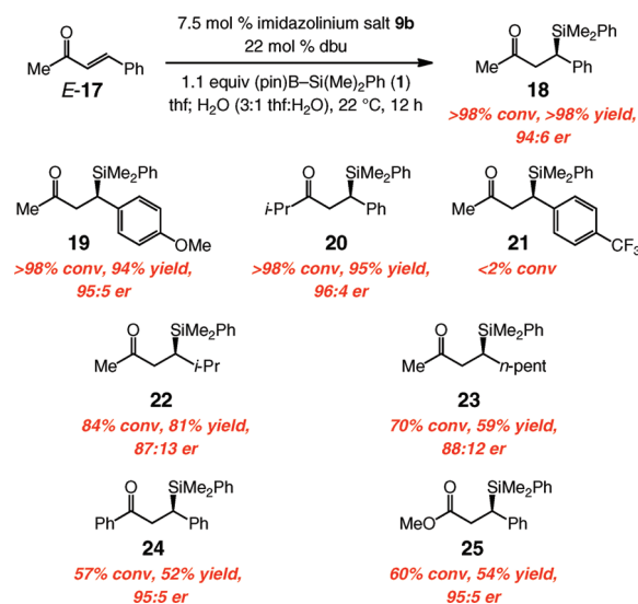
Scheme 3. NHC-Catalyzed Enantioselective Silyl Conjugate Addition (SCA) Reactions with Acyclic \alpha,\beta -Unsaturated Carbonyls a
