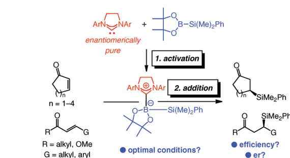
Scheme 1. NHC-Catalyzed Silyl Conjugate Addition to Unsaturated Carbonyls
