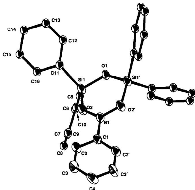
Fig. 2. The molecular structure of 2 showing the labelling scheme used in the text. Primed atoms are related to the unprimed atoms of the asymmetric unit by -x, y, 0.5 - z . Thermal ellipsoids are at the 30% probability level.
