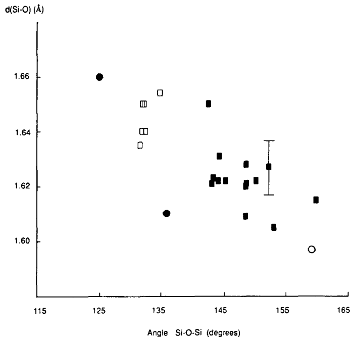
Fig. 3. Plot of d(\text{Si-O}) (Å) against \angle \text{Si-O-Si} (degrees) for \text{Si}_3\text{O}_3 ( \square ) and \text{Si}_4\text{O}_4 ( \blacksquare ) rings. Data are taken from ref. 33. Approximately 90% of the data are within the typical error bar shown (many of the \text{M}_4\text{O}_4 data having much smaller errors); data with larger errors are indicated by ( \bullet ) or ( \circ ) for \text{Si}_3\text{O}_3 and \text{Si}_4\text{O}_4 rings, respectively.
