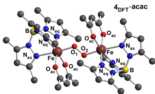
Figure 4. Model of 4-acac derived from DFT geometry optimizations. The computed structure exhibits almost perfect C_{2h} symmetry. Computed bond distances (Å) and angles (deg): Fe–O 1(2) 1.994, Fe–N eq (ave) 2.173, Fe–N ax 2.364, Fe–O ac (ave) 2.037, O 1 –O 2 1.389, Fe \cdots Fe 4.882, Fe–O 1 –O 1 122.8.
