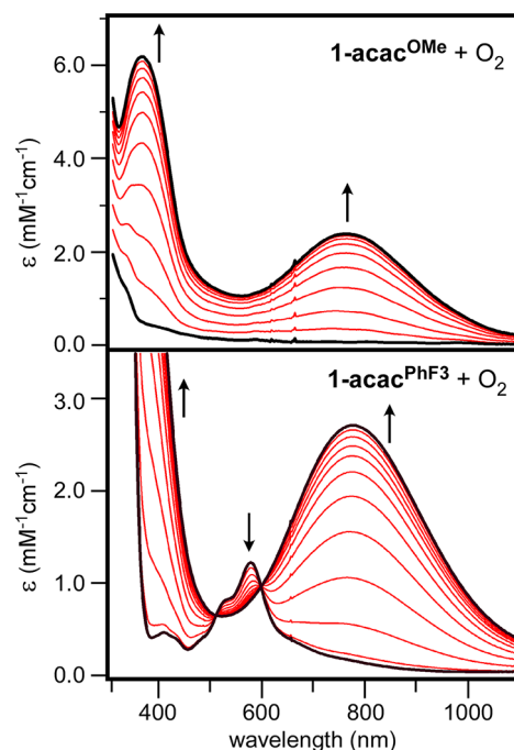
Figure 2. Time-dependent absorption spectra of the reaction of 1\text{-acac}^{\text{OMe}} (top) and 1\text{-acac}^{\text{PhF3}} (bottom) with \text{O}_2 at -70^\circ\text{C} in toluene. The molar absorptivities of the resulting 4\text{-acac}^{\text{X}} intermediates are based on the initial concentrations of the 1\text{-acac}^{\text{X}} precursors.
