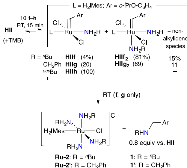
Scheme 3. Reaction of HII with Primary Amines.
