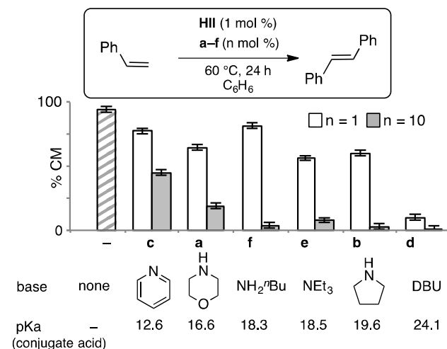
Figure 1. Impact of N -base on metathesis yields. 36
