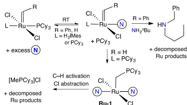
Scheme 1. Amine-Induced Deactivation of the Grubbs Catalysts.
