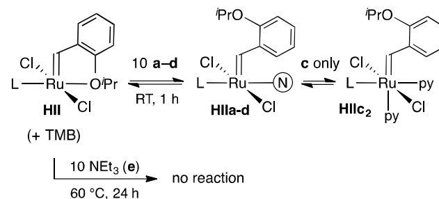
Scheme 2. Reaction of HII with Di- or Trisubstituted N -Donors. a
