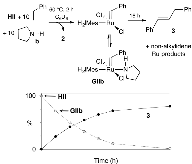
Scheme 6. Reaction of HII with Styrene and Pyrrolidine, and Rate Plot for Loss of Alkylidene.
