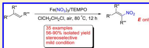
Scheme 2. Nitration of Olefins with \text{Fe}(\text{NO}_3)_3
