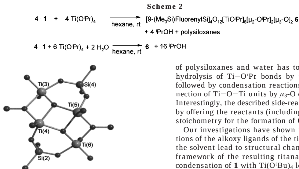
Figure 3. Top view of the upper half of 6 .
