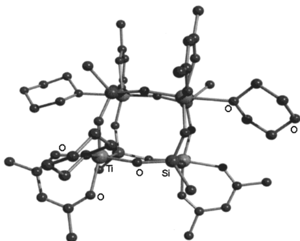
Figure 6. Drawing of the structure of compound 10·4 dioxane. For clarity, Cp* groups are represented by the ipso carbon atom.
