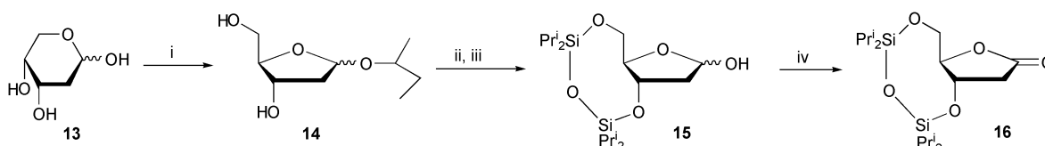
Scheme 3 Reagents and conditions: i, butan-2-ol, HCl, rt, 25 min; ii, Pr 2 Si(Cl)OSi(Cl)Pr 2 , imidazole, THF, rt, 90 min; iii, TFA, H 2 O, CH 2 Cl 2 , –15 °C, 20 min; iv, pyridinium chlorochromate, CH 2 Cl 2 , rt, 16 h.
