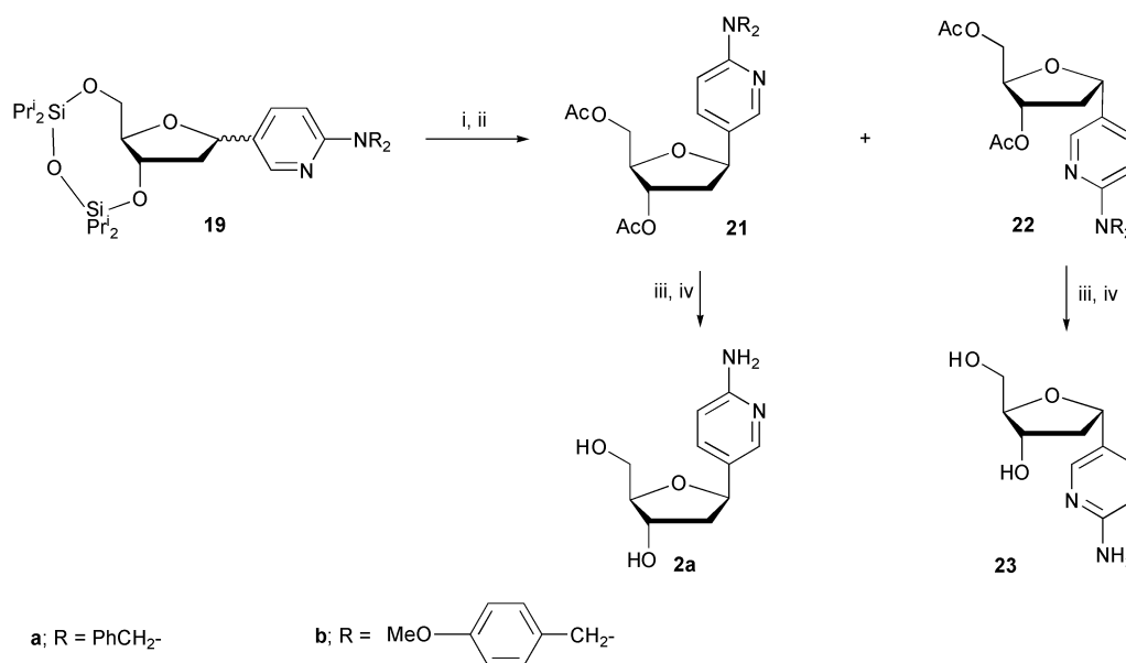
Scheme 5 Reactions and conditions: i, Et 4 NF, MeCN, rt, 90 min; ii, Ac 2 O, 1-methylimidazole, C 5 H 5 N, rt; iii, a (for 21a and 22a ), CAN, MeCN-H 2 O (98 : 2 v/v), rt, 25 min or b (for 21b ) TFA-CH 2 Cl 2 (1 : 1 v/v), reflux, 90 min; iv, MeNH 2 , EtOH, rt, 16 h.
