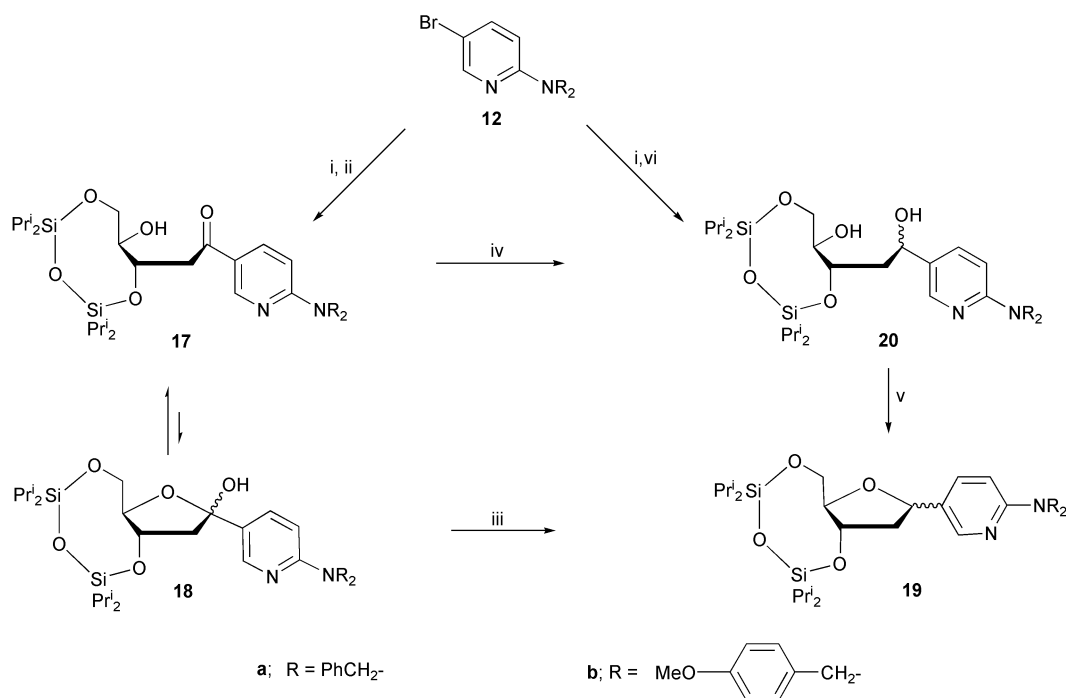
Scheme 4 Results and conditions: i, n BuLi, n -hexane, THF, -78^{\circ}\text{C} , 40 min; ii, lactone 16 , THF, -78^{\circ}\text{C} , 4 h; iii, Et 3 SiH, Et 2 O-BF 3 , CH 2 Cl 2 , -78^{\circ}\text{C} to -10^{\circ}\text{C} , 6 h; iv, NaBH 4 , MeOH, 0^{\circ}\text{C} , 2 h or L-Selectride, THF, -78^{\circ}\text{C} to rt; v, diethyl or diisopropyl azodicarboxylate, Ph 3 P, THF, 0^{\circ}\text{C} , 3 h; vi, lactol 15 , THF, -78^{\circ}\text{C} , 1 h and then -78^{\circ}\text{C} to 0^{\circ}\text{C} over 3 h.
