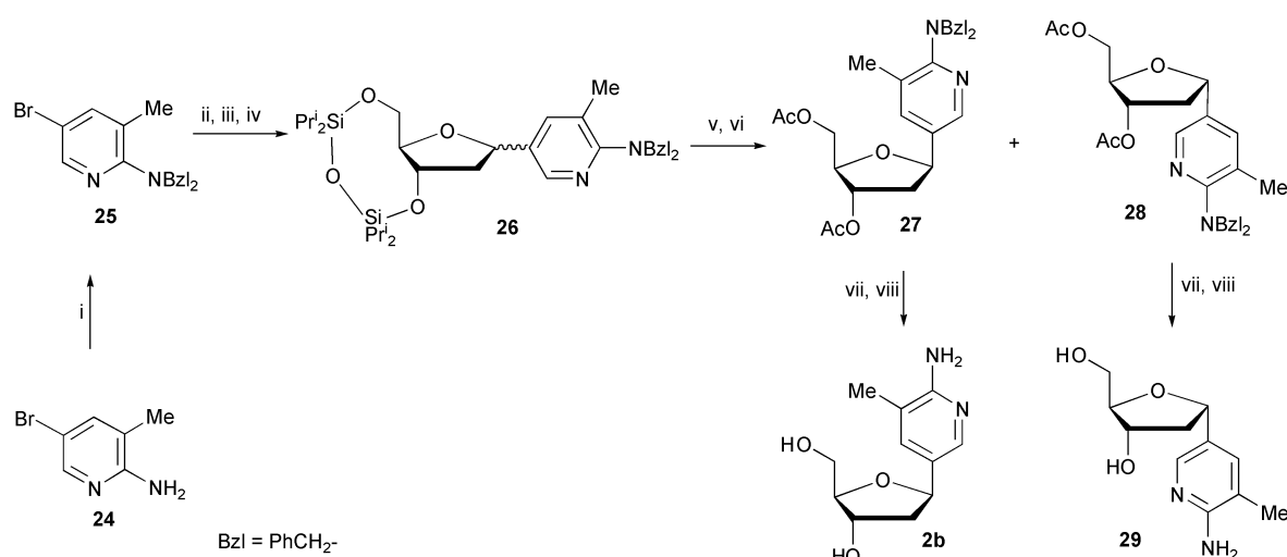
Scheme 6 Reactions and conditions: i, Bzl-Br, NaH, DMA, THF; ii, n BuLi, n -hexane, THF, -78^{\circ}\text{C} , 40 min; iii, lactol 15 , THF, -78^{\circ}\text{C} , 1 h and then -78^{\circ}\text{C} to 0^{\circ}\text{C} over 3 h; iv, diisopropyl azodicarboxylate, \text{Ph}_3\text{P} , THF, 0^{\circ}\text{C} , 3 h; v, \text{Et}_4\text{NF} , MeCN, rt, 90 min; vi, \text{Ac}_2\text{O} , 1-methylimidazole, \text{C}_5\text{H}_5\text{N} , rt; vii, CAN, MeCN– \text{H}_2\text{O} (98 : 2 v/v), rt, 25 min; viii, \text{MeNH}_2 , EtOH, rt, 16 h.
