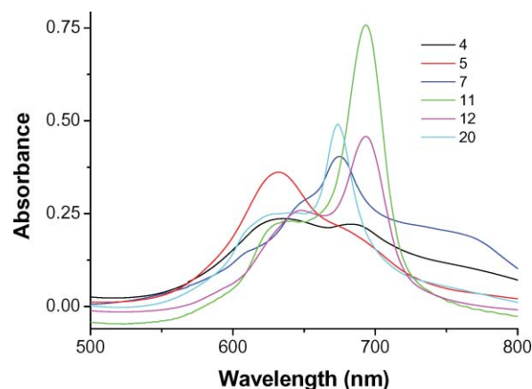
Fig. 3 Electronic absorption spectra of all the glucosylated phthalocyanines, formulated with Cremophor EL, in the DMEM medium. The concentrations of the phthalocyanines were fixed at 8 \mu\text{M} .
