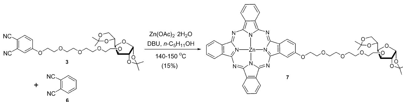
Scheme 2 Synthesis of mono-β-glucosylated phthalocyanine 7 .
