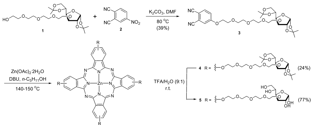
Scheme 1 Synthesis of tetra-β-glucosylated phthalocyanines 4 and 5 .
