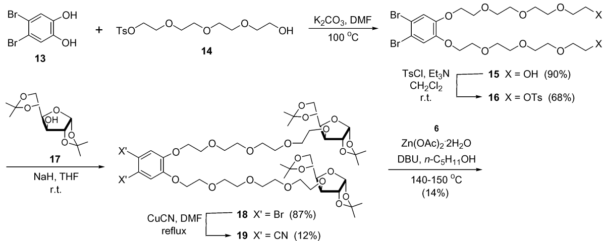
Scheme 3 Synthesis of di- \alpha -glucosylated phthalocyanines 11 and 12 .
