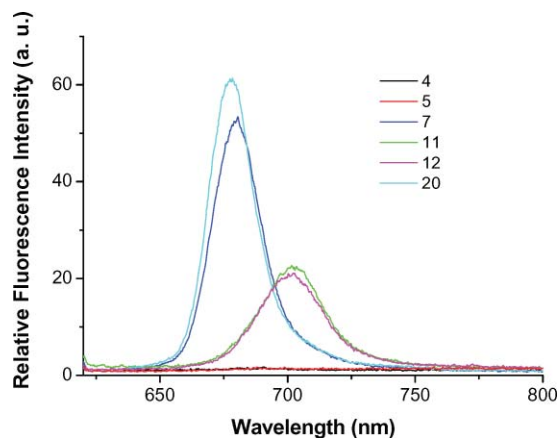
Fig. 4 Fluorescence spectra of all the glucosylated phthalocyanines, formulated with Cremophor EL, in the DMEM medium. The concentrations of the phthalocyanines were fixed at 8 \mu\text{M} .
