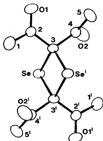
Fig. 1. ORTEP diagram of [\text{Se}(\text{acac})]_2 showing the numbering scheme employed. Atoms not otherwise indicated are carbon atoms. Primed atoms are related to those given in Table 1 by -x, -y, -z .
