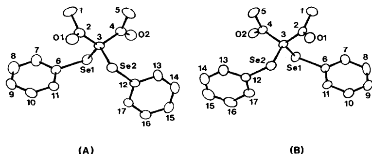
Fig. 2. ORTEP diagram of the two molecules, A and B, of [\text{PhSe}]_2[\text{acac}] showing the approximate mirror relationship. Atoms not otherwise indicated are carbon atoms.
