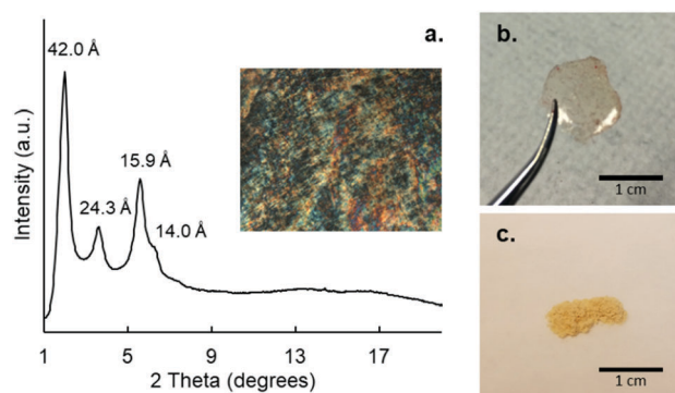
Fig. 2 (a) PXRD spectrum and POM image (inset, 5× mag.) of the TEMPO-based H II resin. (b) Photo of the initially prepared TEMPO-based H II resin as a film. (c) Photo of the TEMPO-based H II resin, powdered and sieved for 75–150 μm particle sizes for catalysis experiments.
