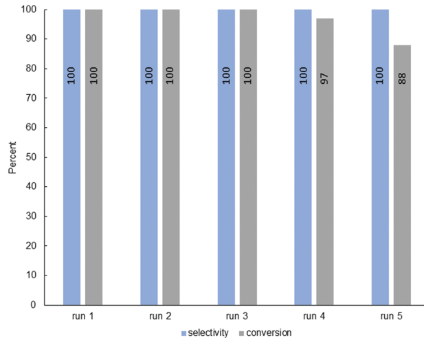
Fig. 4 Percent conversion of BA (gray bars) and percent product selectivity for benzaldehyde (blue bars) after 3 h of reaction for successive recycling experiments using the same TEMPO-based H II resin sample as catalyst. Reaction conditions: 5 mol% available catalyst sites relative to BA with NaNO 2 and I 2 (15 mol%) as co-catalysts in glacial AcOH solvent at 50 °C under 1 atm O 2 .
