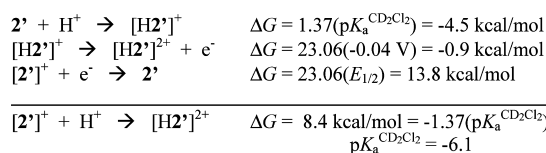
Scheme 2. Bordwell Calculation at 20 °C of the \text{pK}_a^{\text{CD}_2\text{Cl}_2} of [\text{H}2']^{2+} . Assuming E_{1/2} of the [\text{H}2']^{+/2+} Couple as 0.04 V
