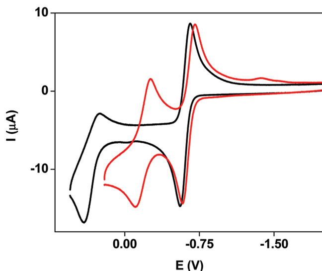
Figure 4. Cyclic voltammograms of a \text{CH}_2\text{Cl}_2 solution of 1 (black) and 2' (red) illustrative of the effect of the azadithiolate on the second anodic event. Conditions: 0.001\text{ M } 2' , 0.300\text{ M } [(\text{C}_4\text{H}_9)_4\text{N}]\text{PF}_6 , \text{CH}_2\text{Cl}_2 , 20\text{ }^\circ\text{C} , 0.1\text{ V/s} scan rate.
