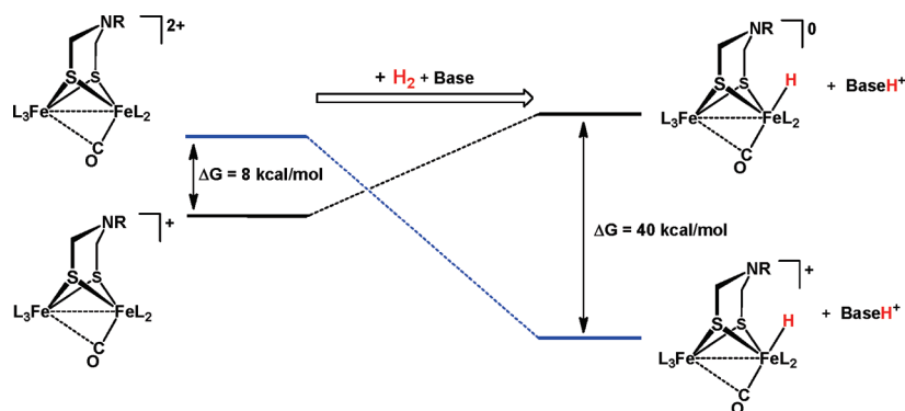
Figure 6. Free energy changes (vs E(\text{Fc}^{0/+}) = 0 V) for the hydrogenation of mixed-valence and diferrous dithiolato complexes using data obtained for [\text{Fe}_2[(\text{SCH}_2)_2\text{NR}](\text{CO})_3(\text{dppv})(\text{PMe}_3)]^n ( n = +, 2+ ). The calculation assumes that the proton binds to a base of \text{pK}_a^{\text{MeCN}} = 10 .
