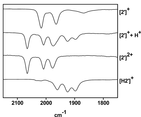
Figure 5. IR spectra ( \text{CH}_2\text{Cl}_2 solution) for [2']^+ (top), the products of its reaction with 0.5 equiv of \text{H}(\text{OEt}_2)_2\text{BARF}_4 (middle top), [2']^+(\text{BARF}_4)_2 (middle bottom), and [\text{H}2']^+ generated by protonation of 2' with \text{H}(\text{OEt}_2)_2\text{BARF}_4 (bottom). Component IR bands ( \text{CH}_2\text{Cl}_2 ) are as follows: [2']^+ 2017, 1965, 1867 \text{cm}^{-1} ; [2']^{2+} 2065, 2009, 1977; [\text{H}2']^+ 1960, 1925, 1898 \text{cm}^{-1} .
