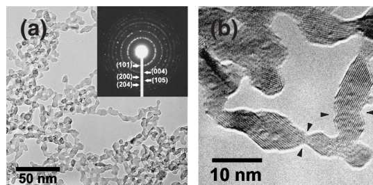
Figure 3. (a) TEM image and (b) HRTEM image of \text{TiO}_2 nano-network structure after reaction at 353 K for 4 days at TIPT:ACA:LAHC = 4:8:1, inset: SAED pattern.
