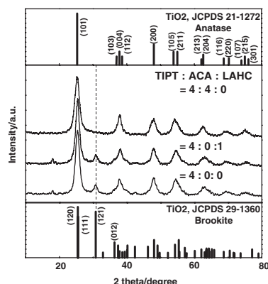
Figure 2. XRD patterns of \text{TiO}_2 nanostructures at TIPT:ACA:LAHC = 4:4:0, 4:0:1 and 4:4:0 after reaction at 353 K for 4 days.
