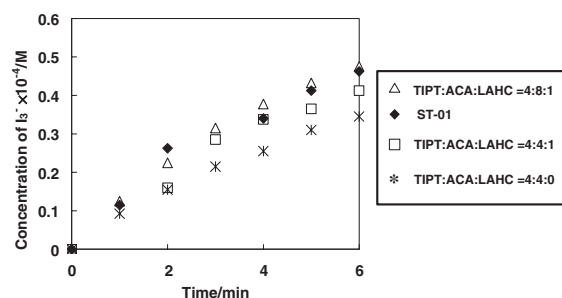
Figure 4. Photocatalytic activity of \text{TiO}_2 nanostructured materials together with ST-01.
