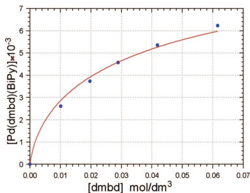
Figure 1. Nonlinear regression fit of the equilibrium concentrations determined by ^1\text{H} NMR technique at 213 K for the reaction [\text{Pd}(\eta^2\text{-fn})(\text{BiPy})] + \text{dmdb} \leftrightarrow [\text{Pd}(\eta^2\text{-dmdb})(\text{BiPy})] + \text{fn} .
