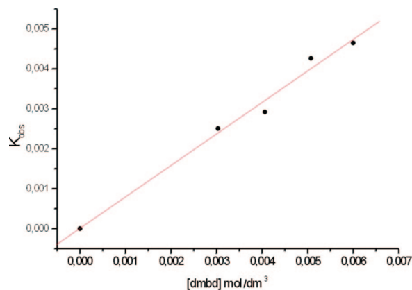
Figure 2. Linear regression plot of k_{\text{obs}} vs [\text{dmdb}]_0 for the reaction of complex 2a with dmdb.
