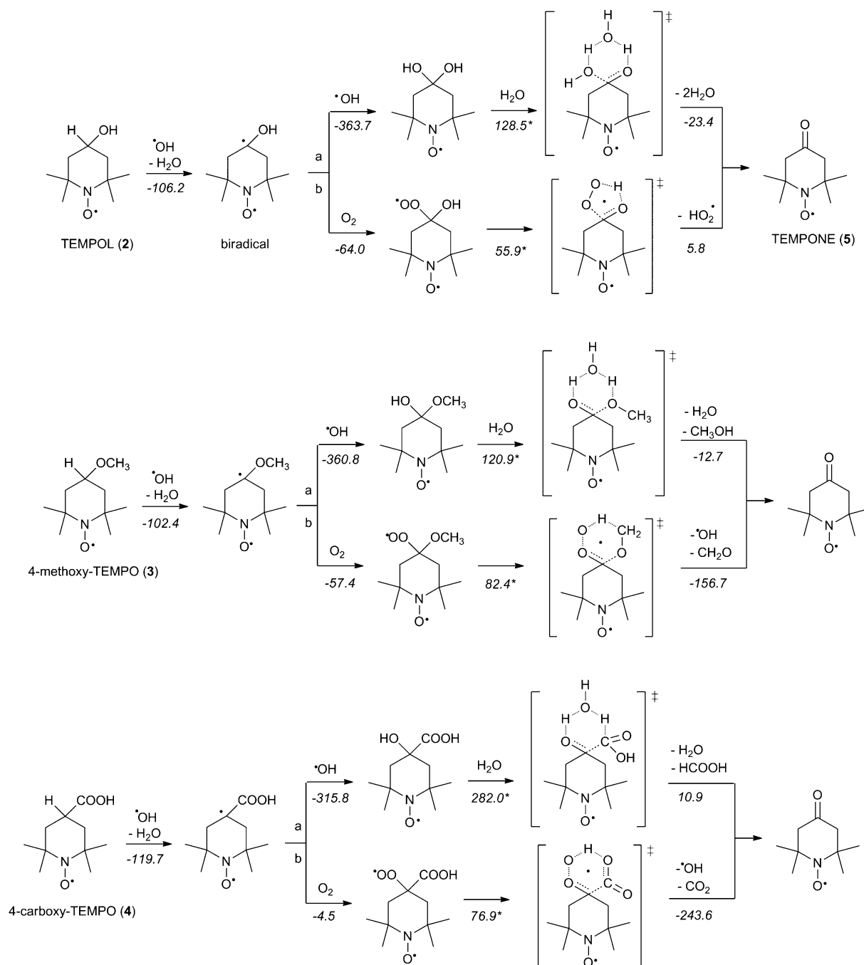
Scheme 4 After formation of a biradical by H^+ abstraction, (a) the product from recombination with HO\cdot can rearrange to TEMPONE through a 6-membered cyclic transition state with a water molecule to facilitate hydrogen transfer. (b) Alternatively, addition of O_2 to the biradical yields a peroxy radical, which forms TEMPONE by intramolecular hydrogen transfer. Values in italics (in \text{kJ mol}^{-1} ) correspond to gas-phase Gibbs free reaction energies and activation barriers (denoted by an asterisk).
