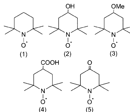
Fig. 1 TEMPO derivatives used as HALS model compounds:
