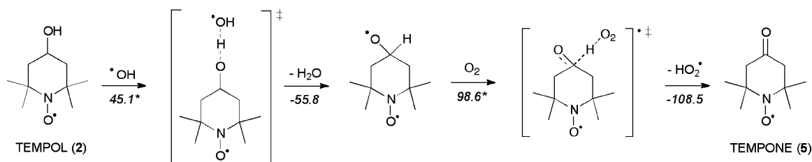
Scheme 5 Alternative pathway to TEMPONE 5 from TEMPOL 2 via an alkoxy radical, which subsequently adds to O _2 and eliminates HO _2\cdot . Values in italics (in \text{kJ mol}^{-1} ) correspond to gas-phase Gibbs free reaction energies and activation barriers (denoted by an asterisk).
