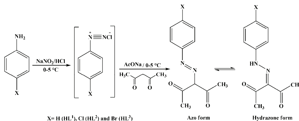
Scheme 1. Synthesis of 3-(arylhydrazono)acetylacetone derivatives (HL).
