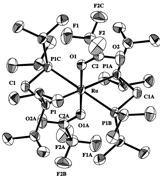
Fig. 3. Molecular structure (ORTEP diagram) of compound 7 . Selected bond lengths (Å) and bond angles (°): Ru–P1 2.3938(8), Ru–O1 2.121(3), O1–C2 1.260(6), O2–C2 1.213(6); P1–Ru–P1C 71.14(4), P1–Ru–P1B 108.86(4), P1–Ru–P1A 180.0, O1–Ru–O1A 180.0.
