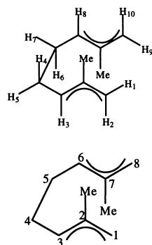
Fig. 4. Assignment of protons and carbon atoms of the octadienediyl ligand of compounds 16 and 17 .
