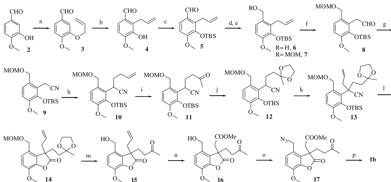
Scheme 1. Reagent and conditions: (a) Allyl bromide, K_2CO_3 , acetone, 4 h, 96%; (b) 200^\circ C , 6 h, 85%; (c) TBSCl, imidazole, CH_2Cl_2 , 4 h, 90%; (d) NaBH_4 , MeOH, 85%; (e) MOMCl, DIPEA, CH_2Cl_2 , 8 h, 85%; (f) OsO_4 , 2,6-lutidine, NaIO_4 , 1,4-dioxane/water, 28 h, 81%; (g) NH_2OH \cdot HCl , pyridine, then CuSO_4 , Et_3N , DCC, CH_2Cl_2 , 5 h, 87%; (h) homoallyl bromide, LDA, DMPU, THF, -78^\circ C , 2 h, 93%; (i) PdCl_2 , CuCl, O_2 , DMF/ H_2O , 12 h, 92%; (j) ethyleneglycol, pTSA , benzene, 80^\circ C , 6 h, 88%; (k) allyl bromide, LDA, DMPU, THF, -78^\circ C , 2 h, 94%; (l) (i) 3 N KOH, C_2H_5OH , reflux, 0.5 h; (ii) aq solution of NaHSO_4 till pH 5, 86% for two steps; (m) 4 N HCl-THF, 2 h, 94%; (n) (i) O_3 , CH_2Cl_2 , -78^\circ C , 5 min, then (CH_3)_2S ; (ii) NaClO_2 , NaH_2PO_4 , 2-methyl-2-butene, acetonitrile–water, 56% for two steps; CH_2N_2 , (C_2H_5)_2O , 5 min, quantitative; (o) DPPA, DBU, toluene, 80^\circ C , 18 h, 92%; (p) Zn, NH_4Cl , EtOH, 80^\circ C , 5 min, 26%.
