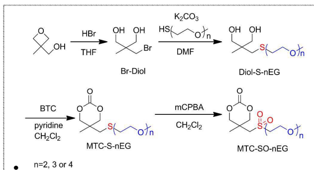
Scheme 1. Synthetic routes for MTC-S-nEG and MTC-SO-nEG.
