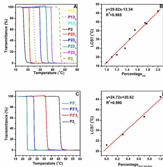
Figure 6. (A) Turbidity measurement for aqueous solution of polycarbonates with different ratios of MTC-SO-nEGs (3 g/L in aqueous solution). (B) Plot of LCST as a function of the percentage of EG unit in copolymer. (C) Turbidity measurement for aqueous solution of polycarbonates with different ratios of MTC-SO-4EG to MTC-S-4EG (3 g/L in aqueous solution). (D) Plot of LCST as a function of the percentage of MTC-SO-4EG in copolymer.
