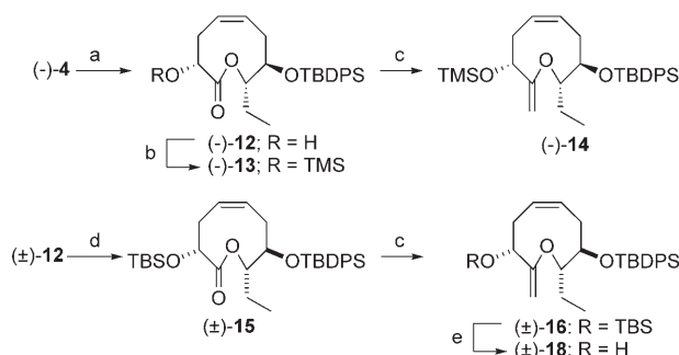
Scheme 3. Enolate oxidation and methylenation. a) KHMDS, THF, –78°C then ( \pm )-2-(phenylsulfonyl)-3-phenyloxaziridine, then ( \pm )-camphor-10-sulfonic acid, 79%; b) TMSCl, Et 3 N, THF, 98%; c) Tebbe reagent, DMAP, THF, –40°C, RT, 90% (–)- 14 , 94% (±)- 16 ; d) TBSCl, imidazole, DMF, 98%; e) TBAF, THF, 29–38%. DMAP=4-dimethylaminopyridine; KHMDS=potassium hexamethyl disilazide; TBAF=tetrabutylammonium fluoride; TBS= tert -butyldimethylsilyl; TMS=trimethylsilyl.
