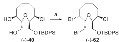
Scheme 15. Synthesis of the dibromide (-)-62 . a) \text{CBr}_4 , \text{P}(\text{Oct})_3 , toluene, 70^\circ\text{C} , 90%.
