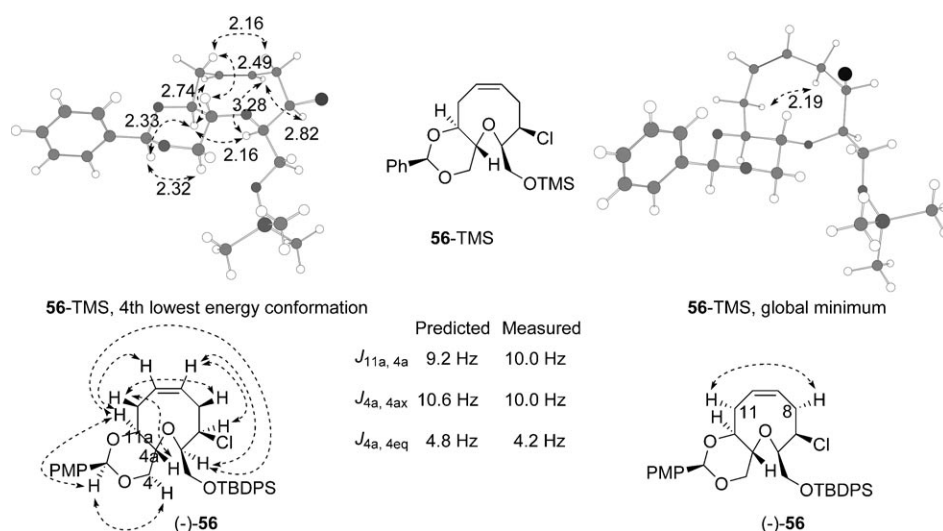
Figure 6. Conformations of 56-TMS corresponding to the acetal (-)-56 . The distances on the molecular model are in Ångströms (Å). Selected ^1\text{H} NMR NOEs are shown on structure (-)-56 . Coupling constants were calculated by using the Altona equation.
