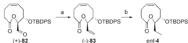
Scheme 20. Synthesis of the lactone ent - 4 —formal synthesis of non-natural (-)-obtusenyne ent - 1 . a) \text{MePPh}_3\text{Br} , KHMDS, THF 98%; b) \text{Pd/C} , \text{H}_2 , \text{EtOH} , 67%.
