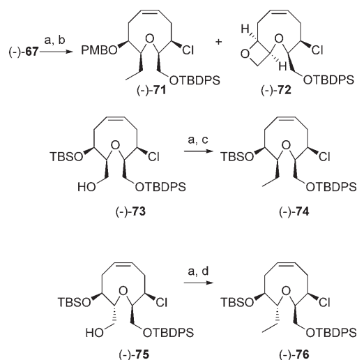
Scheme 18. Cuprate displacement studies. a) \text{TiF}_4 , pyridine, \text{CH}_2\text{Cl}_2 , -20^\circ\text{C} ; b) \text{Me}_2\text{CuLi} , \text{Et}_2\text{O} , 0^\circ\text{C} , 34% (-)- 71 , 34% (-)- 72 ; c) \text{Me}_2\text{CuLi} , \text{Et}_2\text{O} , 0^\circ\text{C} , 65–73% from (-)- 73 ; d) \text{Me}_2\text{CuLi-LiCN} , \text{Et}_2\text{O} , 0^\circ\text{C} , 36% from (-)- 75 .
