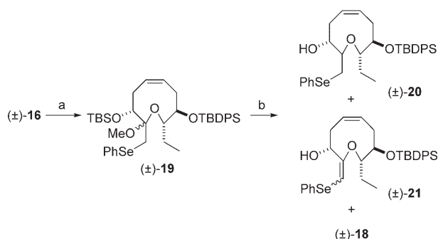
Scheme 4. Methoxy selenation and reduction. a) PhSeCl, i\text{Pr}_2\text{EtN} , MeOH, \text{CH}_2\text{Cl}_2 , 55%; b) DIBAL, \text{CH}_2\text{Cl}_2 , RT, 20% (±)-20, 24% (±)-21, 12% (±)-18.
