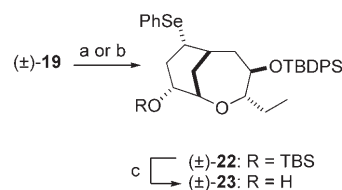
Scheme 5. Formation of the 2-oxabicyclo[4.3.1]decane (±)-23. a) \text{TiCl}_4 , \text{Et}_3\text{SiH} , -78^\circ\text{C} , then MeOH, 59% (±)-23; b) \text{TiCl}_4 , \text{Et}_3\text{SiH} , -78^\circ\text{C} , then \text{NH}_4\text{Cl} , 79% (±)-22; c) TBAF, THF, RT, 68%.
