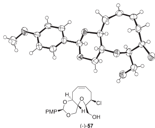
Figure 7. X-ray crystal structure of the acetal (-)-57 . The X-ray crystal structure of (-)-57 has two different conformers in the unit cell. One of the conformers shows some disorder in the hydroxymethyl side chain (see the Supporting Information for details).
