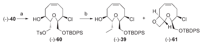
Scheme 14. Synthesis of the \Delta^5 -hexahydrooxonines (-)-39 and (-)-61 . a) TsCl, DMAP, \text{Et}_3\text{N} , \text{CH}_2\text{Cl}_2 , 51% (-)-60 , 24% (-)-40 ; b) \text{Me}_2\text{CuLi-LiCN} , \text{Et}_2\text{O} , -78^\circ\text{C} \rightarrow \text{RT} , 30% (-)-39 , 70% (-)-61 .
