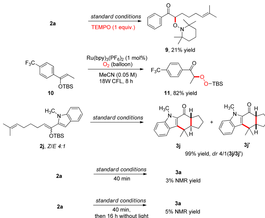
Scheme 5. Mechanistic Studies
