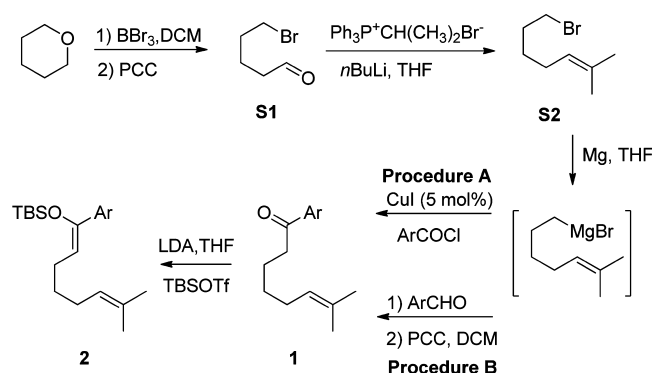
Scheme 3. Synthesis of Silyl Enol Ether 2
