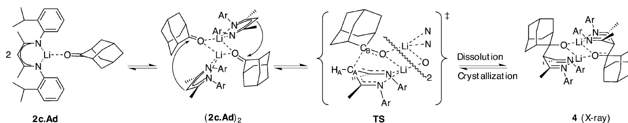
Scheme 5
