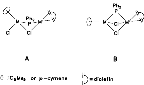
Fig. 1. The doubly-bridged structure A and the triply-bridged structure B .
