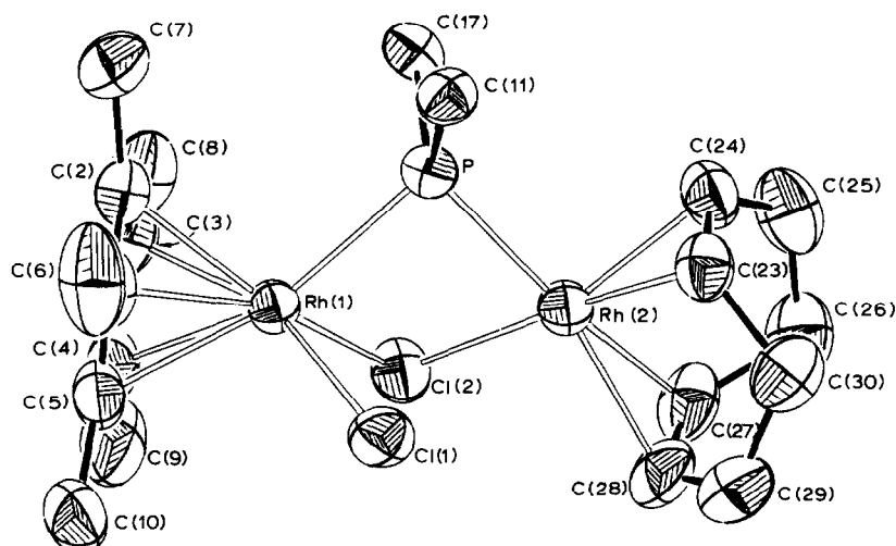
Fig. 2. An ORTEP plot of the structure of [(C_5Me_5)ClRh(\mu-Cl)(\mu-PPh_2)Rh(COD)] (XXI) showing the atomic numbering scheme. Only the ipso carbons of the phenyl groups are shown for clarity.
