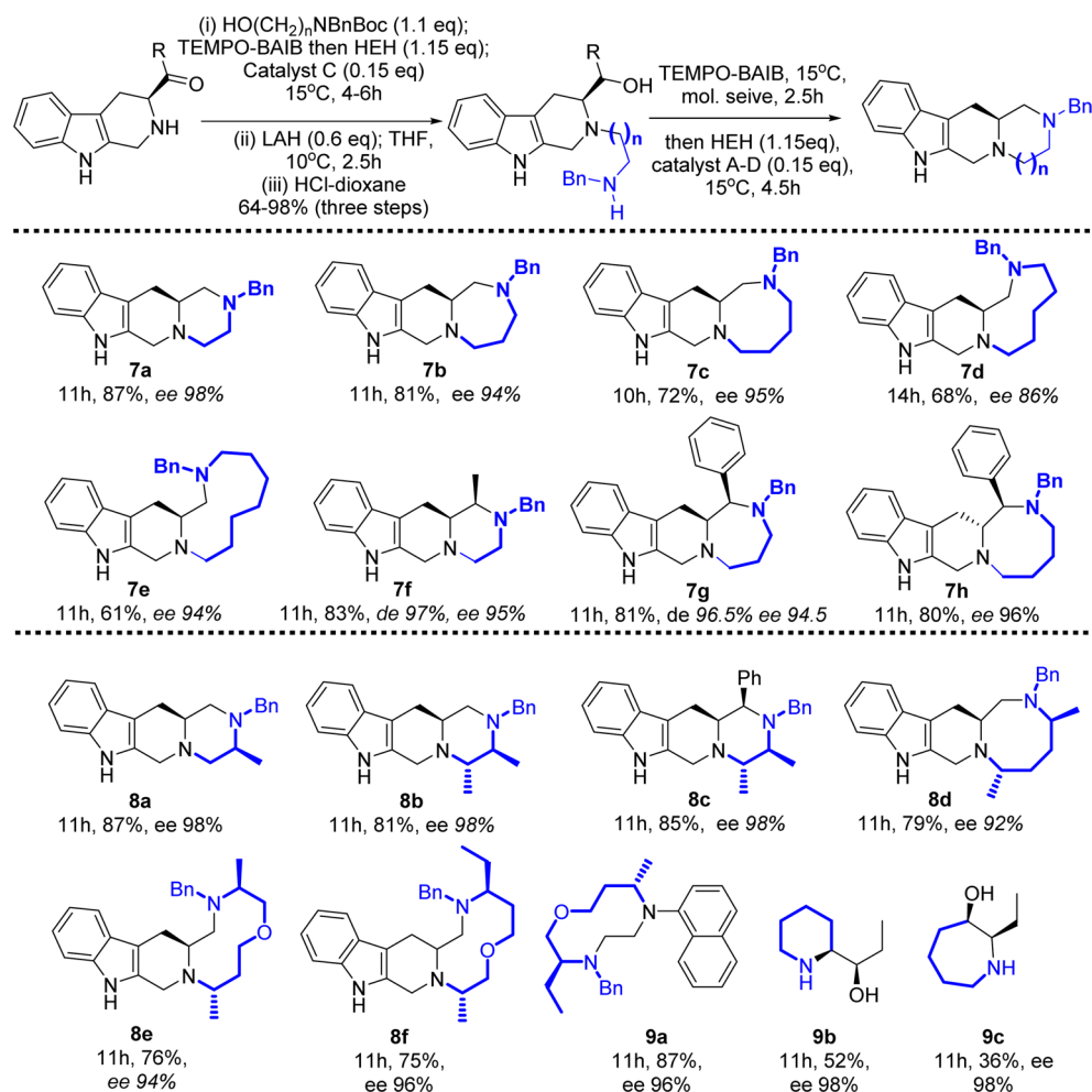
Figure 4. Preparation of octahydropyrazinopyridindoindoles (oHPPs) and their higher ring analogues.
