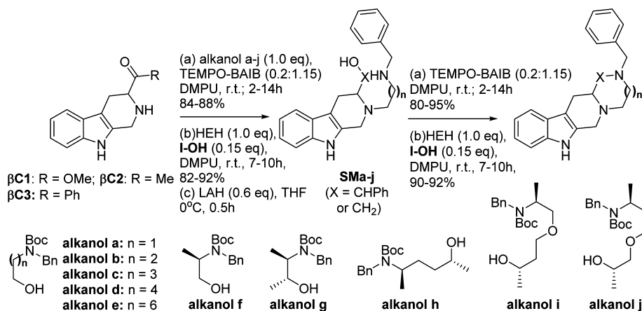
Scheme 3. Representative Scheme Used for the Synthesis of Compounds 7a–h and 8a–f
