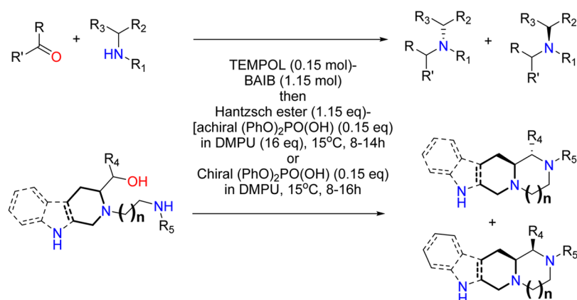
Scheme 1. General Representation of Oxidation/Imine–Iminium Formation Cascade in Both Possibilities of Intramolecular Coupling
