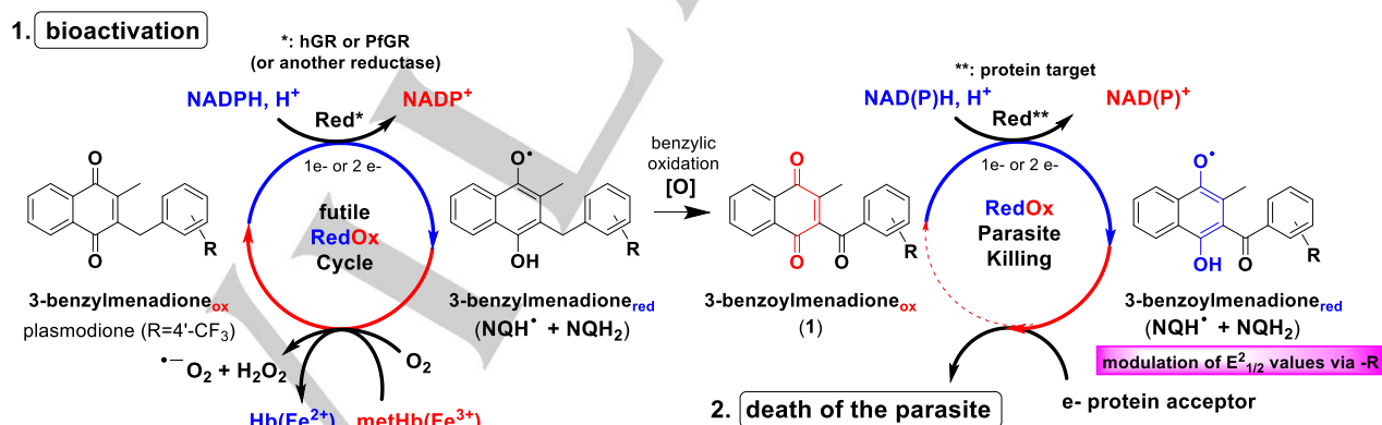
Scheme 10. Proposed mechanism of action of antimalarial 3-benzoylmenadione prodrugs generating toxic 3-benzoylmenadione 1 metabolites in P. falciparum -parasitized red blood cells. The first one-electron transfer leading to the semi-quinone \text{NQH}^{\cdot+} is proposed to be involved in the drug bioactivation (step 1.) while the second one-electron transfer leading to the dihydro-naphthoquinone \text{NQH}_2 might be responsible for parasite killing (step 2). For the sake of clarity, only the 1-e - -reduced NQ species were drawn. Abbrev.: hGR: human glutathione reductase; PfGR: P. falciparum glutathione reductase.
