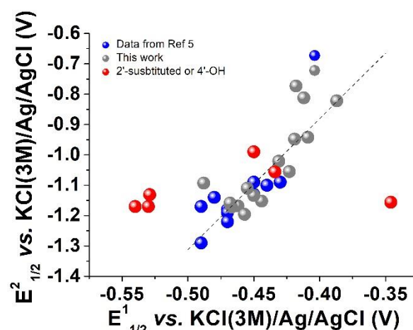
Figure 4. Variation of E_{1/2}^2 (V, second redox step) as a function of E_{1/2}^1 (V, first redox step). \nu = 200 mV s -1 ; reference electrode = KCl(3 M)/Ag/AgCl; working electrode = glassy carbon disk of 0.07 cm 2 area; auxiliary electrode = Pt wire. The dashed line is only provided as a guide for the eyes. ● Data taken from ref [5] . ● Data from this present work. ● Compound with particular behaviour (e.g. 2'-substituted or 4'-OH benzoylmenadiones, see text).
