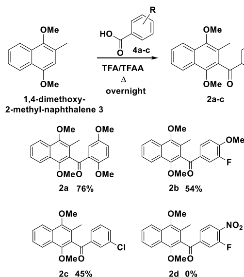
Scheme 5. Preliminary study on the Friedel-Crafts reaction to build 2-acylated 3-methyl-1,4-dimethoxy-naphthalene derivatives 2a-c .
