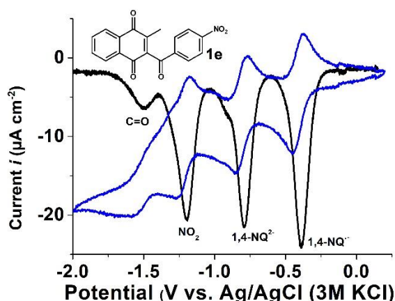
Figure 3. CV (blue) and SWV (black) profiles of 1e (1.40 mM) measured in DMSO with 0.1 M n -Bu 4 PF 6 electrolyte support at 25°C. \nu = 50 mV s -1 ; reference electrode = KCl(3 M)/Ag/AgCl; working electrode = glassy carbon disk of 0.07 cm 2 area.
