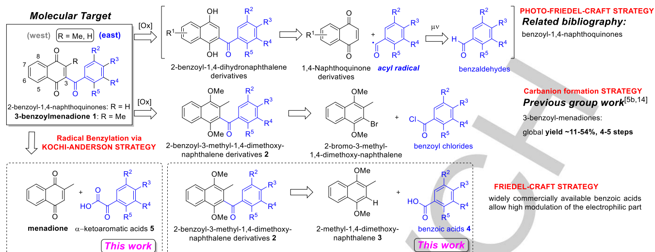
Scheme 1. Synthesis of 3-benzoylmenadione derivatives 1 ( R = \text{Me} ) starting from 1,4-dimethoxy-2-methyl-naphthalene 3 and benzoic acids 4 .
