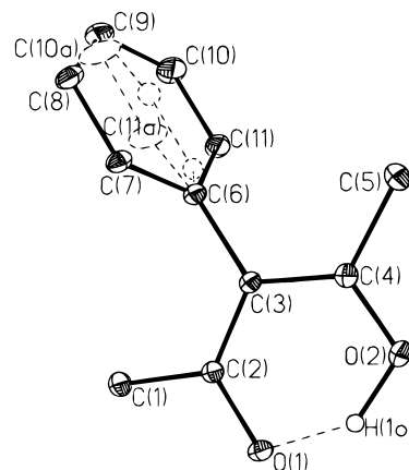
Figure 3. Molecular structure of 3-phenyl-2,4-pentanedione with numbering scheme. The atoms C(7), C(8), C(10), and C(11) are disordered in two positions (a) (50% probability level).
